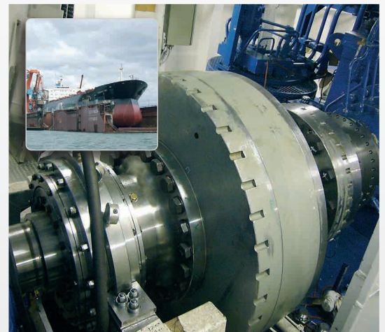
Engines, gearboxes and propeller shafts on ships are aligned using Easy-Laser® system. Thanks to versatile brackets you can install the equipment in the most appropriate place; shaft, coupling or flywheel.
