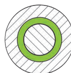
The lubricating film in a bearing is very thin. A machine poorly aligned, or a foundation not supporting the machine in a proper way, will cause increased pressure and overheating of the lubricating film. This will in the end destroy the lubricant, and cause the machine to fail.
