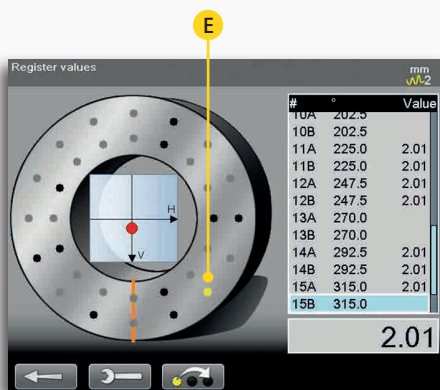
The point to be measured is indicated in the image. It is also possible to see from the display screen whether the laser beam hits the detector.
