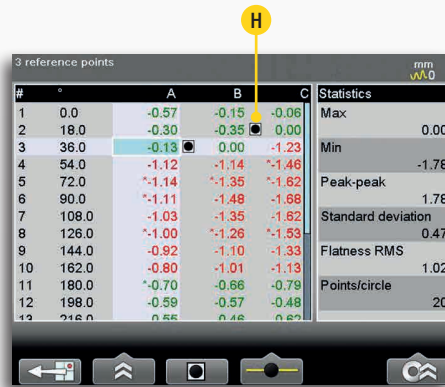
Result table with reference points marked (H). Red values are out of tolerance.
